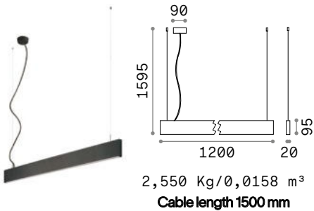
LED SMD Up-light included - Driver 1-10V included
