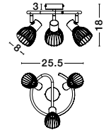
FIUMICINO - 770012 Matt Black Metal LED E14 3x5 Watt 230 Volt IP20 Bulb excluded D: 25.5 H: 18 cm
