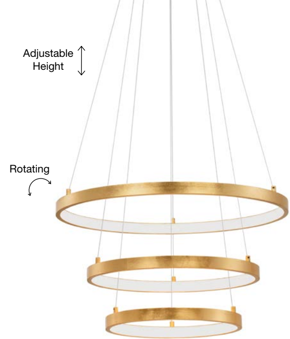
LEON - 9501430 Triac Dimmable Gold Leaf Aluminium & Acrylic LED 83 Watt 230 Volt 5597Lm 3000K IP20 D1: 61 D2: 45 D3: 35.5 H: 150 cm
