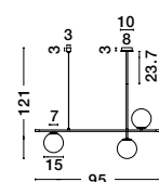
GIT - 9009295 Matt Black & Gold Metal Opal Glass LED G9 2x5 Watt 230 Volt IP20 Bulb Excluded Included Two parts Of Metal 23.7 cm Each Part L: 95 W: 15 H1: 73.5 H2: 121 cm
