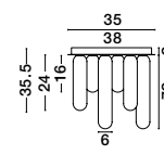
GUSTAVE • 9028854 Light Smoky Grey Glass & Matt Black Metal LED G9 6x5 Watt 230 Volt IP20 Bulb Excluded L: 38 W: 7 H: 35.5 cm
