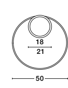
FULINE . 9348072 Triac Dimmable Sandy White Aluminium & Acrylic LED 32 Watt 230 Volt 2320Lm 3000K IP20 D: 50 H: 5 cm
