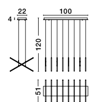
ELETTRA - 9081803 Triac Dimmable Sandy Black Aluminium LED 60 Watt 220-240 Volt 2400Lm 3000K IP20 L: 100 W: 51 H: 120 cm
