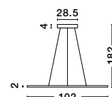
ODERICK - 9100145 Sandy Black Aluminium & Acrylic LED 44 Watt 230 Volt 1346Lm 3000K IP20 D: 102 H: 182 cm
