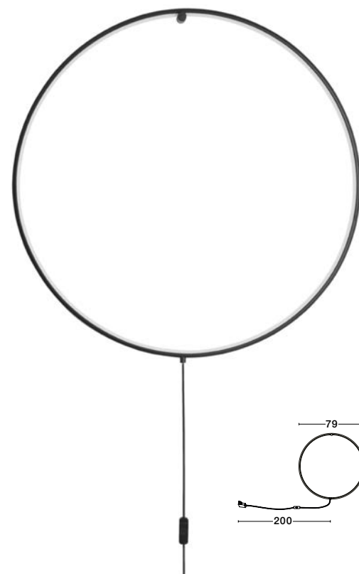
RING - 9108311 Sandy Black Aluminium & Acrylic Black Fabric Wire LED 30 Watt 230 Volt 1445Lm 3000K IP20 D: 79 W: 2 cm Cable Length: 200 cm
