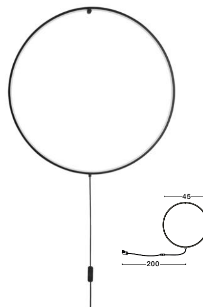
RING - 9108312 Sandy Black Aluminium & Acrylic Black Fabric Wire LED 19 Watt 230 Volt 901Lm 3000K IP20 D: 45 W: 2 cm Cable Length: 200 cm
