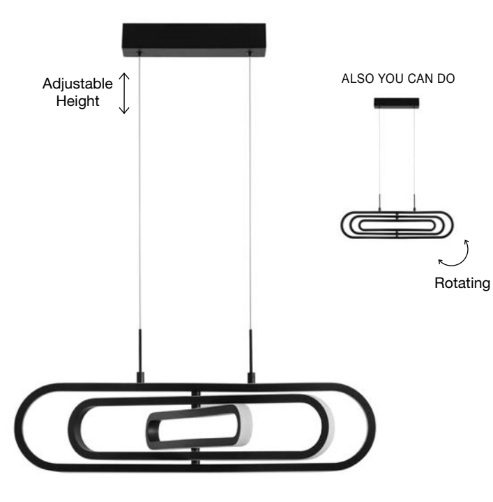
ARTE - 9110351 Triac Dimmable Matt Black Aluminium & Acrylic LED 56 Watt 230 Volt 4441Lm 3000K IP20 L: 64 W: 44 H1: 25.8 H2: 120 cm
