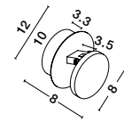
OTTO - 9139805 Sandy White Metal & Aluminium Acrylic LED 5 Watt 230 Volt 469Lm 3000K IP20 D: 12 W: 8 H: 12 cm
