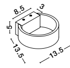
ENNA - 9102461 Sandy White Aluminum & Acrylic LED 6 Watt 230 Volt 444Lm 3000K IP20 L: 13.5 W: 13.5 H: 5 cm
