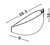
ASTRID - 9128320 Sandy White Metal & Acrylic LED 20 Watt 230 Volt 1183Lm 3000K IP20 L: 28.5 W: 9 H: 16 cm
