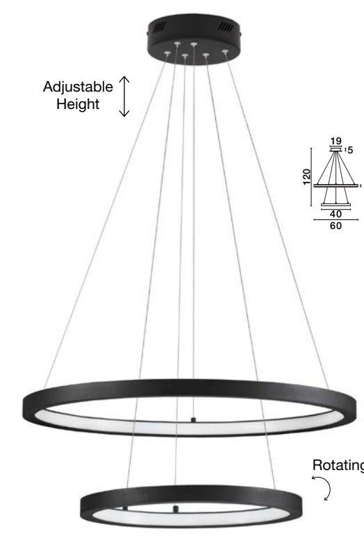
EMPATIA - 9172864 Triac Dimmable Sandy Black Aluminium & Acrylic LED 60 Watt 230 Volt 1755Lm 3000K IP20 D1: 60 D2: 40 H: 120 cm LED WARM WHITE DRIVER INCL.
