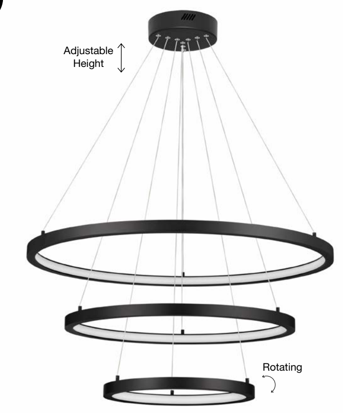
EMPATIA - 9172867 Triac Dimmable Sandy Black Aluminium & Acrylic LED 108 Watt 230 Volt 2245Lm 3000K IP20 D1: 80 D2: 60 D3: 40 H: 120 cm LED WARM WHITE DRIVER INCL.
