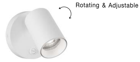
NET - 9011921 Sandy White Aluminium Switch On/Off LED GU10 1x10 Watt IP20 220-240 Volt Bulb Excluded D: 5.7 H1: 9 H2: 10.5 cm
