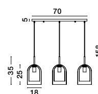
VELOR . 9236740 Double Layered Dark Champagne Glass Black Cord Black Metal Base LED E27 3x12 Watt 230 Volt IP20 Bulb Excluded L: 70 W: 18 H: 158 cm
