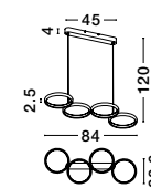
MAGNUS • 9248117 Triac Dimmable Sandy Black Aluminium & Acrylic LED 41 Watt 230 Volt 2300Lm 3000K IP20 L: 84 W: 32 H: 120 cm
