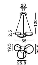
MAGNUS • 9248116 Triac Dimmable Brass Gold Aluminium & Acrylic LED 28 Watt 230 Volt 1900Lm 3000K IP20 D: 55 W: 51.5 H: 120 cm
