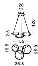
MAGNUS • 9248115 Triac Dimmable Sandy Black Aluminium & Acrylic LED 28 Watt 230 Volt 1900Lm 3000K IP20 D: 55 W: 51.5 H: 120 cm
