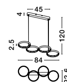
MAGNUS • 9248118 Triac Dimmable Brass Gold Aluminium & Acrylic LED 41 Watt 230 Volt 2300Lm 3000K IP20 L: 84 W: 32 H: 120 cm
