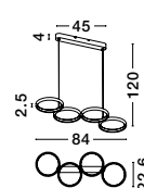
MAGNUS • 9248118 Triac Dimmable Brass Gold Aluminium & Acrylic LED 41 Watt 230 Volt 2300Lm 3000K IP20 L: 84 W: 32 H: 120 cm
