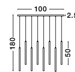
TRIMLE . 9287935 Sandy Black Aluminium & Acrylic LED 21 Watt 230 Volt 1581Lm 3000K IP20 L: 100 W: 8 H: 180 cm
