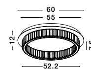
AURELIA - 9333080 Triac Dimmable Gold Metal & Crystal LED 41W 230 Volt 2505Lm 3500K IP20 Class I D: 60 H: 12 cm LED WARM WHITE DRIVER INCL.
