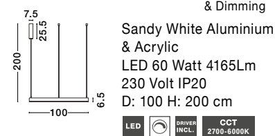
MOTIF - 9190755 · 3000K Triac Dimmable 9530211 · 2700-6000K Changing CCT & Dimming
