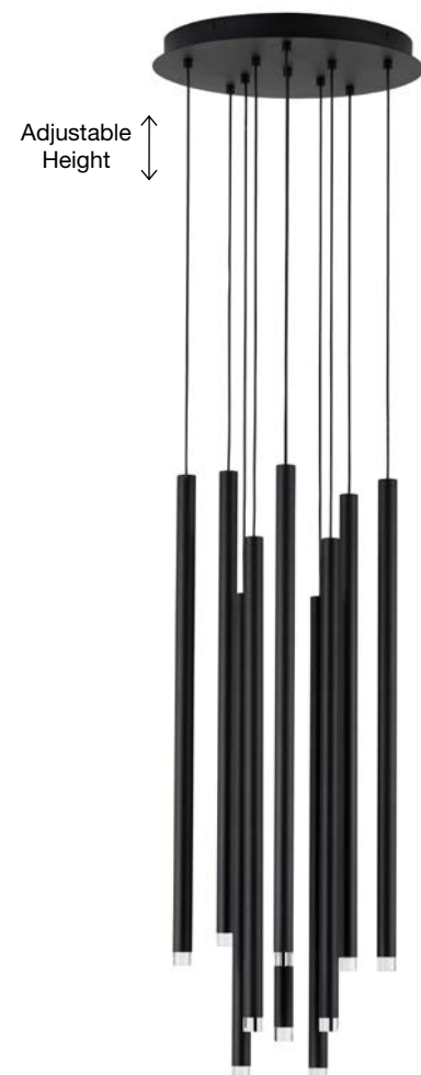
DANDIA - 9540204 Triac Dimmable Black Aluminum LED 69 Watt 220-240 Volt 4223Lm 3000K IP20 D: 40.5 H: 150 cm
