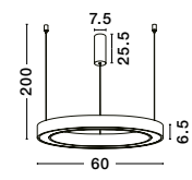
STING - 9558601 Triac Dimmable Sandy Black Aluminium & Acrylic LED 40 Watt 230 Volt 2153Lm 3000K IP20 D: 60 H: 200 cm
