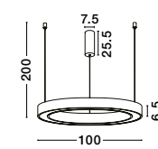
STING - 9558607 Triac Dimmable Sandy Black Aluminium & Acrylic LED 60 Watt 230 Volt 3389Lm 3000K IP20 D: 100 H: 200 cm
