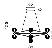
BELINDA • 9695300 Triac Dimmable Black Aluminium & Acrylic LED 42 Watt 230 Volt 2238Lm 3000K IP20 D: 83 W: 46 H: 120 cm
