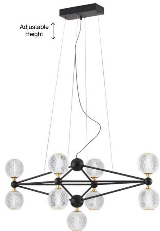
BELINDA • 9695300 Triac Dimmable Black Aluminium & Acrylic LED 42 Watt 230 Volt 2238Lm 3000K IP20 D: 83 W: 46 H: 120 cm
