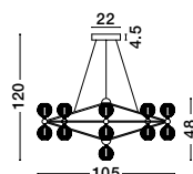
BELINDA • 9695500 Triac Dimmable Black Aluminium & Acrylic LED 78 Watt 230 Volt 4492Lm 3000K IP20 D: 105 H: 120 cm
