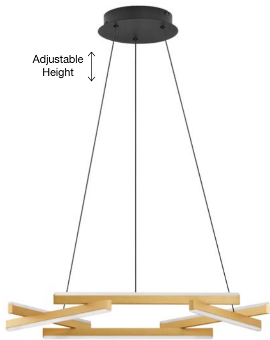
HYDE • 9005652 Triac Dimmable Brushed Gold & Black Aluminium & Acrylic LED 38 Watt 220-240 Volt 2046Lm 3000K IP20 D: 66 H: 150 cm LED WARM WHITE DRIVER INCL.
