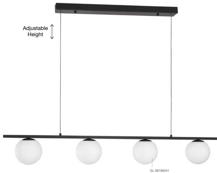
JOLINE - 9919604 Sandy Black Metal & Aluminium White Opal Glass LED 26 Watt 240 Volt 1870Lm 3200K IP20 L: 72 W: 12.5 H: 120 cm 120 33 12.5 72 LED WARM WHITE DRIVER INCL.
